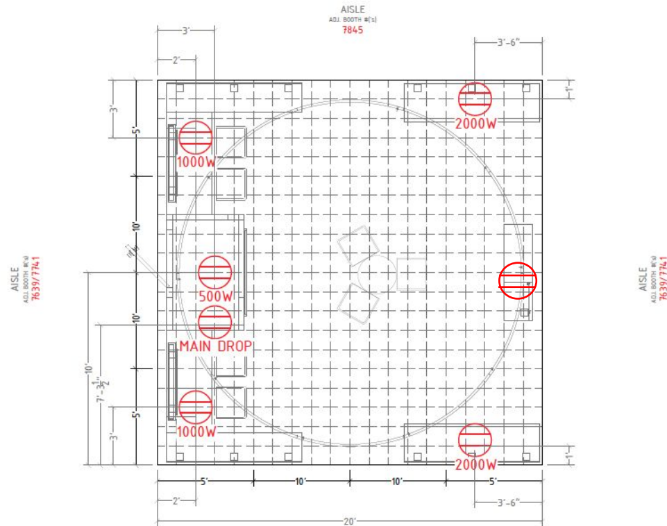
ELECTRICAL FLOOR PLAN SCALE: 1/4" = 1'-0"
